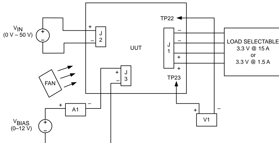
Figure 3. Basic Lab Configuration
